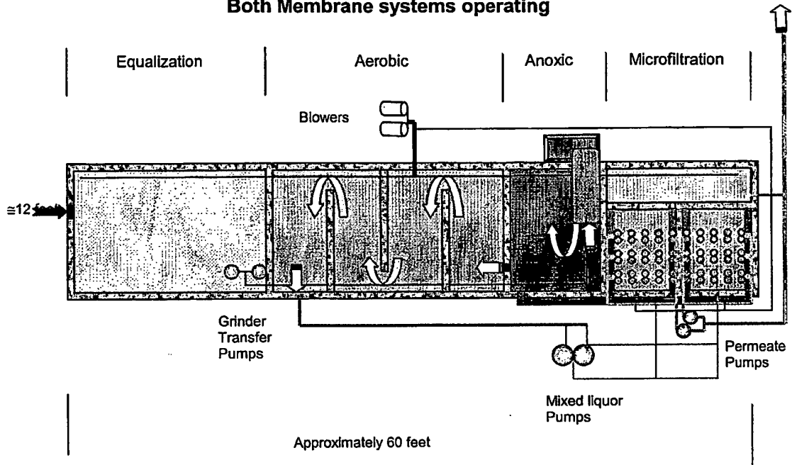
Figure 16 - Operating Mode Both Membrane systems operating
